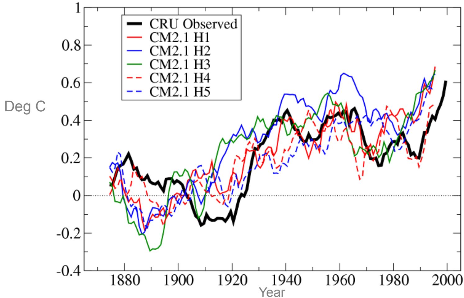
GFDL CM2.1 Historical Forcing Runs Using 5 “Random” Initial Conditions
